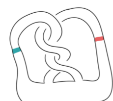
Figure 4: Two band-moves for 9_{46} .
