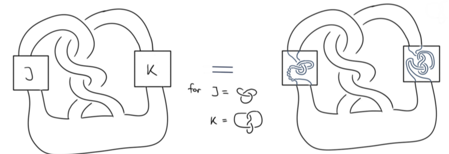
Figure 5: The boxes labelled with J and K indicate that the strands going through them are tied into the knots J and K (all parallel to each other). The extra full twists on the left arise from untwisting the writhe of the projection of the trefoil J .
